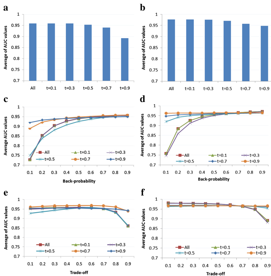
Figure 4 Investigation of the performance of each method on different functional similarity protein complex networks extracted with different thresholds (t). (a) , (c) and (e) are the performance of NBH, RWR and PRINCE for networks which are extracted from SharedGOTermComNet , respectively; (b) , (d) and (f) are the performance of NBH, RWR and PRINCE for networks which are extracted from SharedPPIComNet , respectively. For RWR and PRINCE, back-probability and trade-off parameters were varied in a range of [0.1, 0.9], respectively. Vertical axis represents average AUC values over 270 disease phenotypes. “All” is the original functional similarity protein complex networks (i.e., SharedGOTermComNet in (a) , (c) and (e) ; SharedPPIComNet in (b) , (d) and (f) ).
